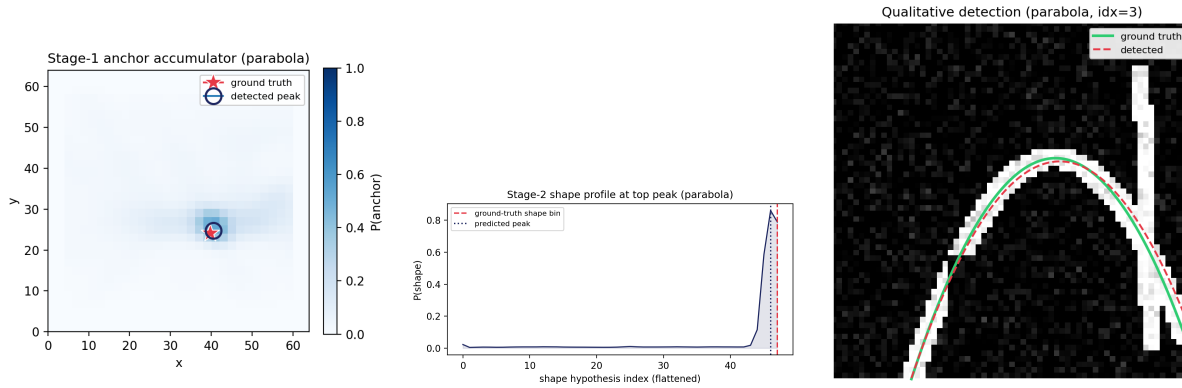
Figure 4: Stage-1 anchor accumulator (left), Stage-2 shape profile at the top peak (center), and the resulting detection against ground truth (right), for a representative parabola test image. The anchor peak lands on the true vertex and the shape profile is sharply peaked near the true curvature bin, giving a near-pixel-tight fit.
